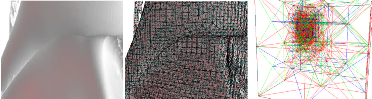
Figure 1: Closeup view of an isosurface feature in the mixing interface of two gases showing the texture mapped surface, underlying triangle mesh, and the adaptively refined tetrahedral mesh around the region of interest. Time step = 273, Isovalue = 206, Isosurface error = 1.5, 50K Triangles, rendered at 7 frames per second.
